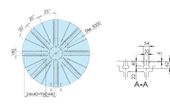
TKV-3500 series
