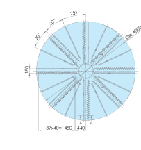
TKV-4500 series
